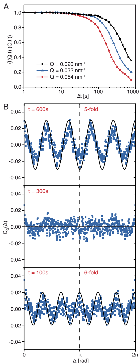
Fig. 2. Temporal relaxation behavior of C_Q(\Delta) and \langle I(Q, t)I(Q, t') \rangle : (A) Normalized temporal intensity autocorrelation function \langle I(Q, t)I(Q, t') \rangle for different Q values (black squares: Q = 0.020 \text{ nm}^{-1} ; blue triangles: Q = 0.032 \text{ nm}^{-1} ; red dots: Q = 0.054 \text{ nm}^{-1} ), \Delta t = t' - t . Solid lines are guide to the eyes. (B) The cross-correlation function C_Q(\Delta) at Q = 0.04 \text{ nm}^{-1} evolves from an initially 6-fold to a 5-fold symmetry. The curves at 600 s and 300 s are averaged over the subsequent 100-s interval; the one at 100 s is averaged over a 50-s interval.
